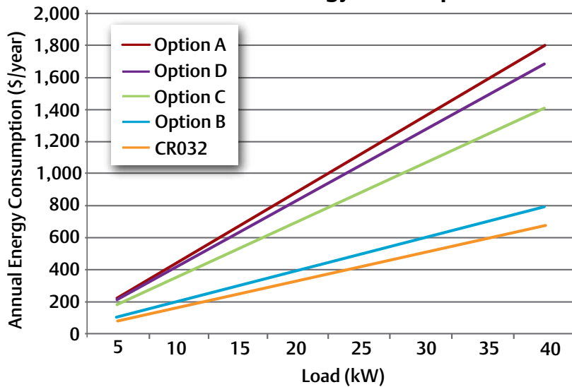
Annual Energy Consumption
