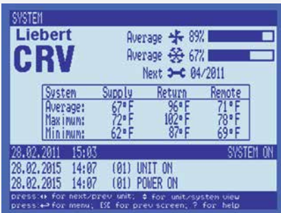
A single view shows the average, minimum, and maximum temperature of every 2T rack sensor in a single- or multi-unit system.
