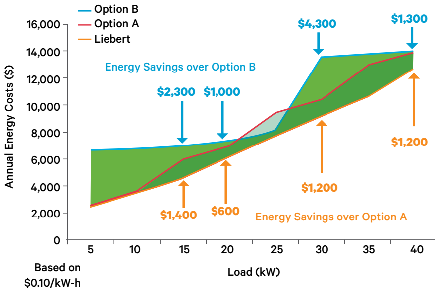
12" DX Row Based Unit Energy Cost Comparison
