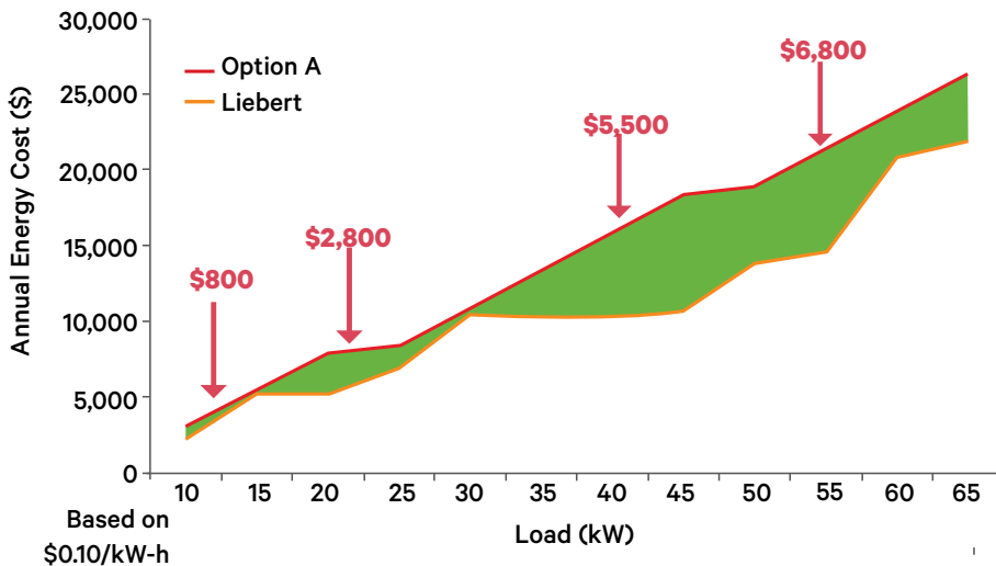
24" DX Row Based Unit Energy Cost Comparison
