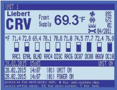
Bar graphs show the inlet temperature of every rack with a 2T temperature sensor.
